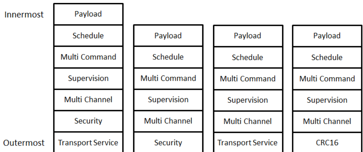
Figure 11, Encapsulation overview
