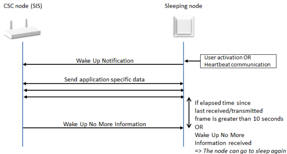
Figure 10, Wake Up Command Class
