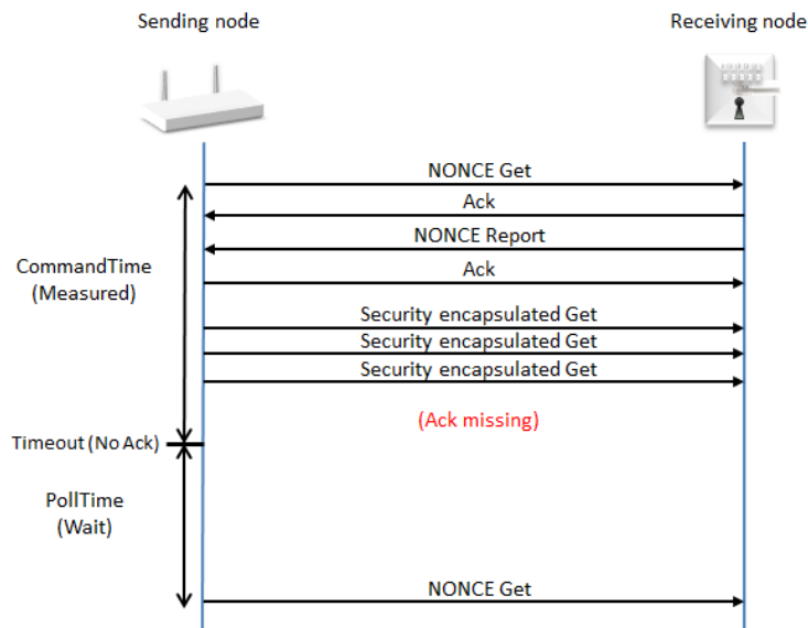
Figure 4, Polling (No Ack, with security 0)
