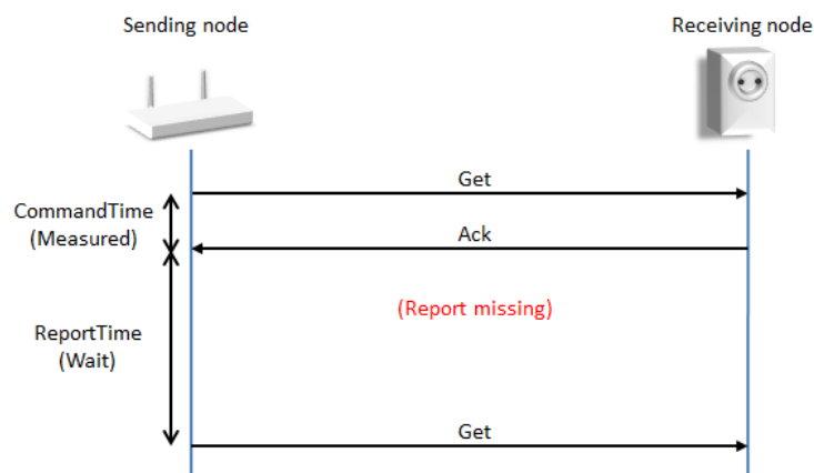
Figure 5, Polling (No Report frame, without security)
