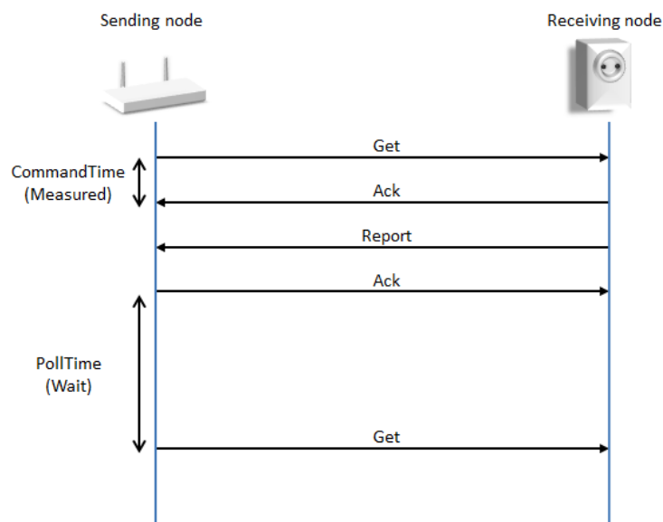
Figure 1, Polling (No errors, without security)
